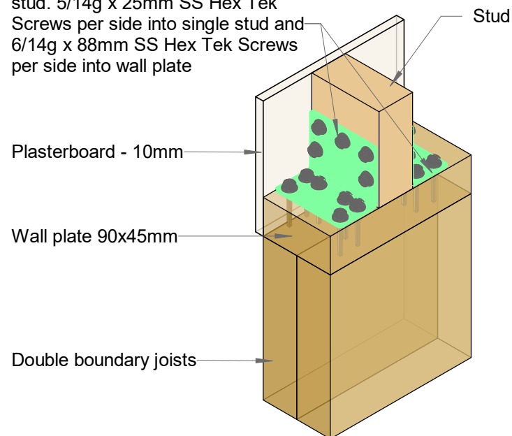
Isometric Detail
